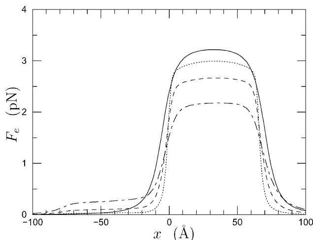
FIGURE 6 Force per elementary (+) charge. The origin of the abscissa lies at the entrance of the IM pore which is 65 Å long. Positive force is directed into the mitochondrion. Solid line is the analytical result (6); computational results are dotted line, r_i = 3 Å; dashed line, r_i = 6.5 Å; and long-dash/short-dash line, r_i = 12 Å.
